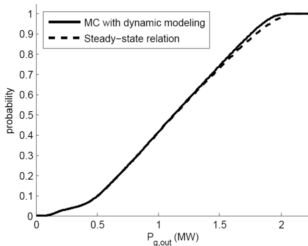
Figure 10: Cumulative distribution function of a 10 turbine wind farm generation obtained with dynamic modeling and steady-state power curve with an annual mean wind speed of 10 m/s.
