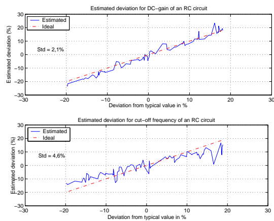
Fig. 6. Estimated deviation (solid) from typical value versus real values for DC-gain (above) and cut-off frequency (below) of an RC circuit. The dashed lines represent the ideal responses.
