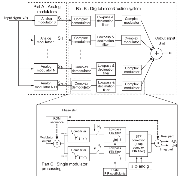
Fig. 1. Extended Frequency Band Decomposition architecture
