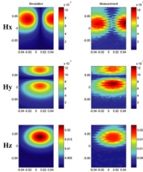
Figure 9. The measured data and the simulated results.
