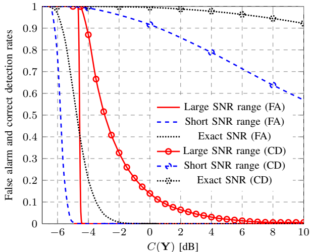
Fig. 3. False alarm (FA) and correct detection (CD) rates for exact, short discrete range \{0, 2.5, 5\} and large discrete range \{-5, -2.5, 0, 2.5, 5\} SNR - M = 1 , N = 8 , L = 10 , SNR = 2.5 dB
