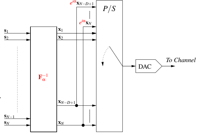
Fig. 1. \alpha -OFDM transmission scheme
