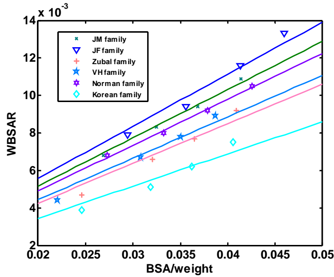
Figure 1: Relationship between BSA/weight and WBSAR at 2100MHz for the families of phantoms.
