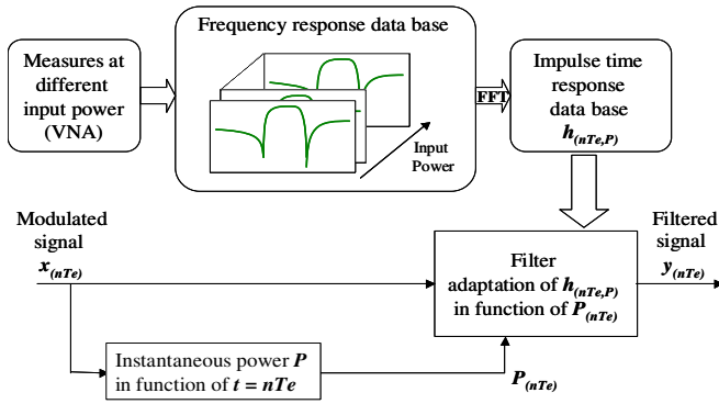
Figure 9 : Principle of the algorithm
