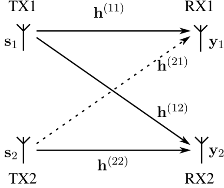
Figure 1 Cognitive interference channel model.
