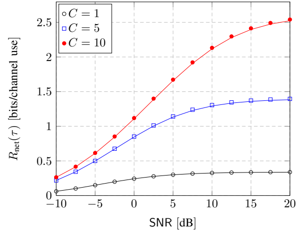
Fig. 3. Net ergodic achievable rate R_{\text{net}}(\tau) vs SNR for \tau = 40 and T = 1000 . The markers are obtained by simulations, the solid lines correspond to the deterministic equivalent \bar{R}_{\text{net}}(\tau) .
