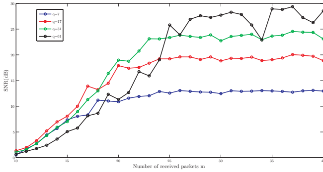
Fig. 4. SNR as a function of the number m of received packets for various field size
