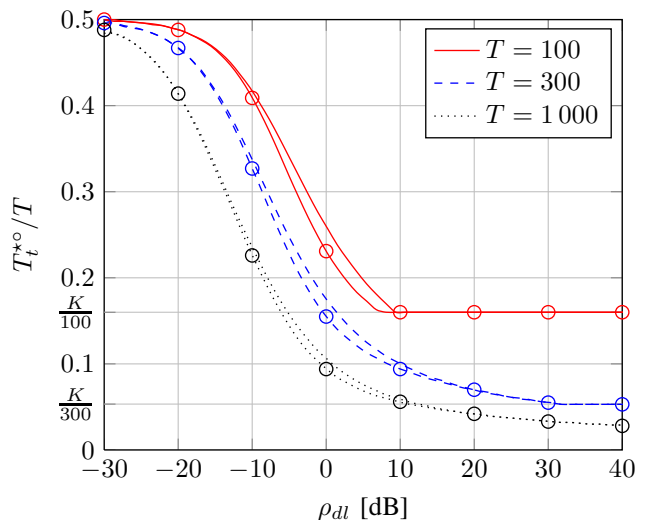
Fig. 13. ZF and RZF-CDA, optimal relative amount of training T_t^{\star\circ}/T vs. \rho_{dl} with M = 32 , K = 16 , \rho_{dl}/\rho_{ul} = 10 , \Theta_k = \mathbf{I}_M \forall k , RZF is indicated by circle marks.
