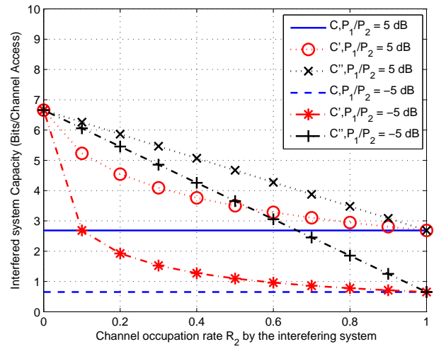
Fig. 10. : Channel capacity in the presence of co-channel interference and noise with respect to the interfering channel occupation rate, for R_1 = 1 , SNR = 20 dB, B_1 = 0.1 , B_2 = 1 and \delta = 0 .
