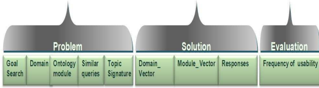
Figure 5. Case Representation.
