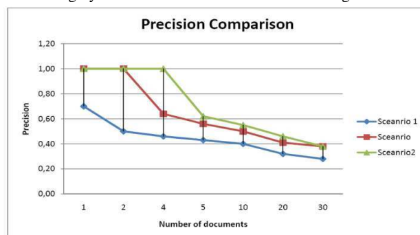
Figure 9. Precision comparison
