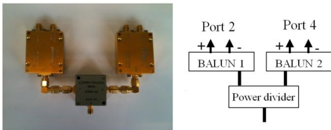
Figure 4. Antenna array excitation circuit composed of two pulse lab PSPL BALUNs and a power divider in the middle of the photography.
