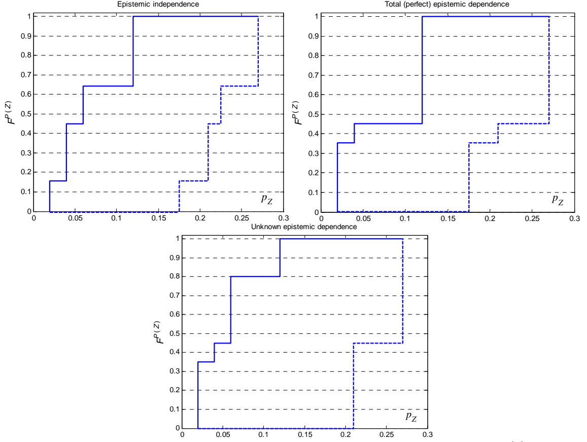
Figure 3. Upper (solid lines) and lower (dashed lines) CDFs, \bar{F}^{P(Z)} and F^{P(Z)} , of the probability (chance) P(Z) of the conjunction of two (objectively) independent events B_1 and B_2 with probabilities (chances) P(B_1) and P(B_2) distributed as in Figure 2, under the assumptions of independence (top left), total (top right) and unknown (bottom) epistemic dependence
