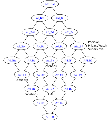
Figure 1. Lattice based on the Data Encryption (A) and Traffic Communication Encryption (B) properties.
