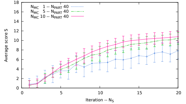
Figure 4: Average scores returned by all the policies during the learning.
