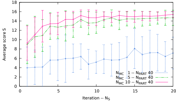
Figure 1: Average scores while testing the policy of the best particle ( N_{\text{PART}} = 40 , N_{\text{MC}} increases).
