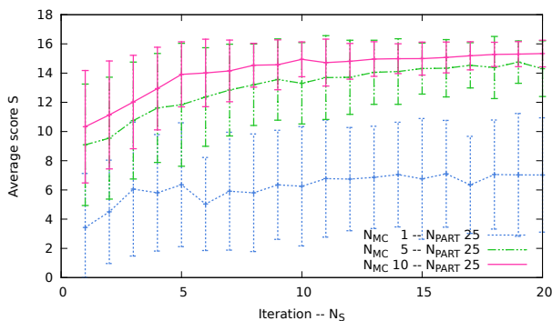
Figure 3: Average scores while testing the policy of the best particle ( N_{\text{PART}} = 25 , N_{\text{MC}} increases).
