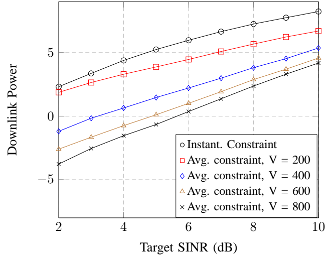
Fig. 1. Average energy expenditure Vs target QoS for a two cell scenario, each cell consisting of two UTs, N_t = 5 , P_{peak} = 10\text{dB} .
