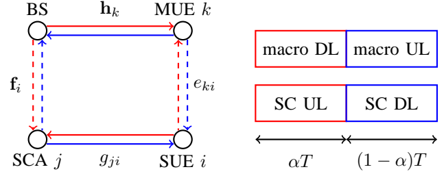
Fig. 3. A two-tier network employing R-TDD protocol; solid arrows denote direct links and dashed arrows denote interfering links.
