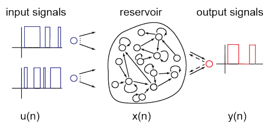
Figure 1: Functional Principle of Echo State Networks, Based on (Jaeger, 2005)
