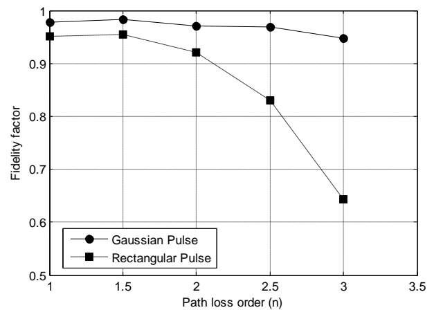
Fig. 10. Fidelity factor versus path loss order.
