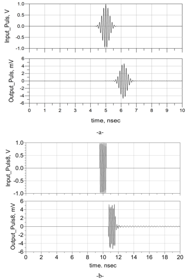
Fig. 9. UWB signals: (a) Gaussian transmitted/received pulses, (b) Rectangular transmitted/received pulses.
