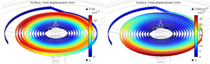
Fig. 3. Displacement of the balance-spring to due (a) magnetostatic forces and (b) magnetostriction effect.
