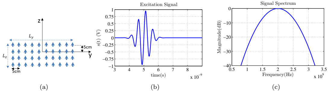
Figure 1: The time-domain excitation signal (b) applied to each of the 40 dipoles composing the AUT (a) and the magnitude of the excitation signal spectrum (c). The maximum of the spectrum is at 2\text{GHz} .
