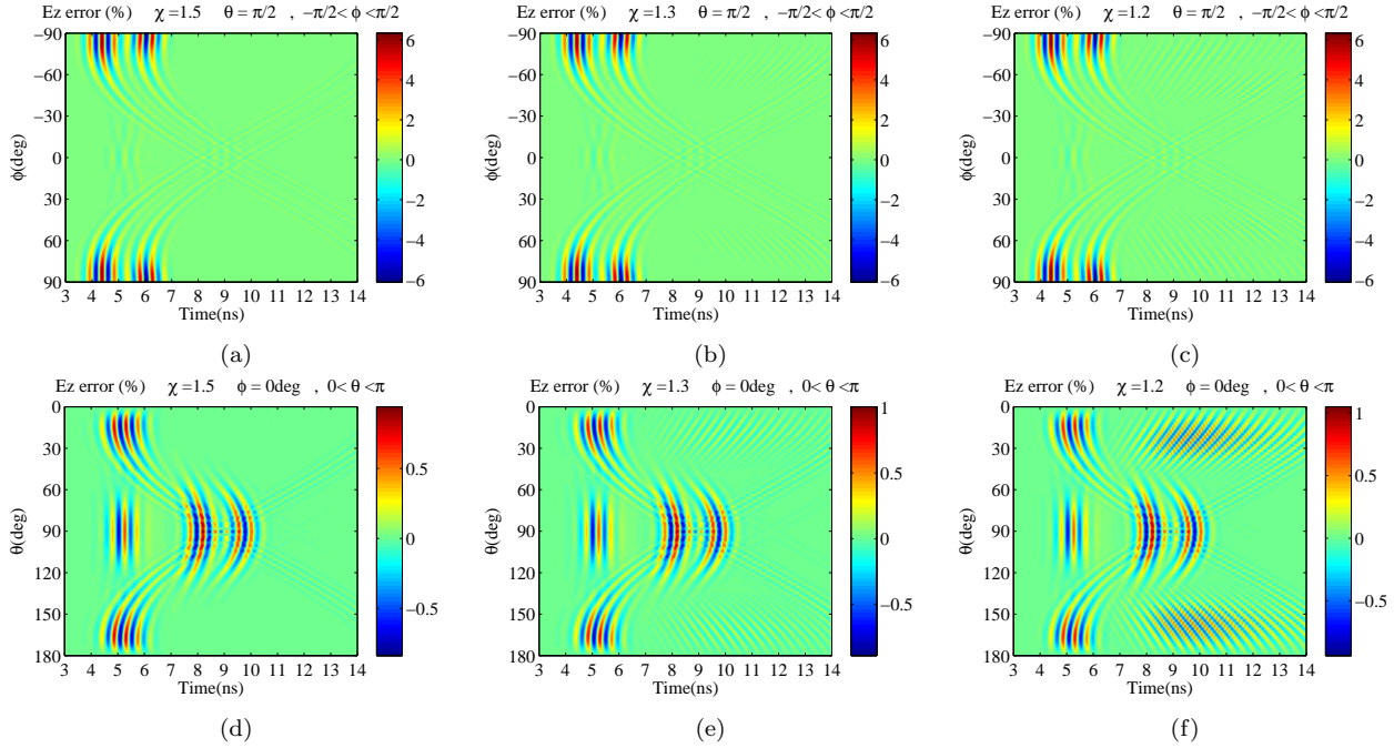
Figure 6: The FF Ez component error as a function of time for the plane cut \theta = \pi/2 . (a) for \chi = 1.5 , (b) for \chi = 1.3 , (c) for \chi = 1.2 . The Ez error as a function of time for the plane cut \phi = 0 , (d) for \chi = 1.5 , (e) for \chi = 1.3 , (f) for \chi = 1.2 .
