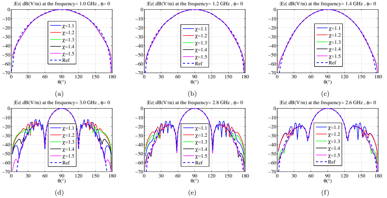
Figure 7: Comparison of far-field Ez-component at the plane cut \phi = 0 with D_{max} = 150cm , x_{meas} = 50cm and \Delta y = \Delta z = \lambda_0/2\chi for \chi = 1.1, 1.2, 1.3, 1.4, 1.5 . (a-d) For 1GHz and 3GHz ( F_{-30dB} ) respectively. (b-e) For 1.2GHz and 2.8GHz ( F_{-20dB} ) respectively. (c-f) For 1.4GHz and 2.6GHz ( F_{-10dB} ) respectively.
