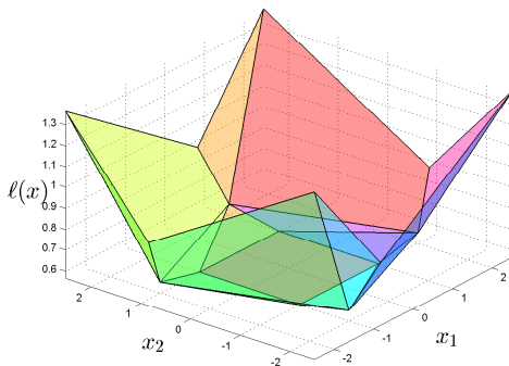
Fig. 6. A convex lifting of the partition in Fig.4.
