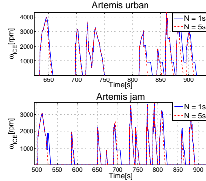
Fig. 6. MPC-based stop-start included, \omega_{ICE} for two values of the prediction horizon: 1s and 5s, respectively; Artemis urban and traffic jam
