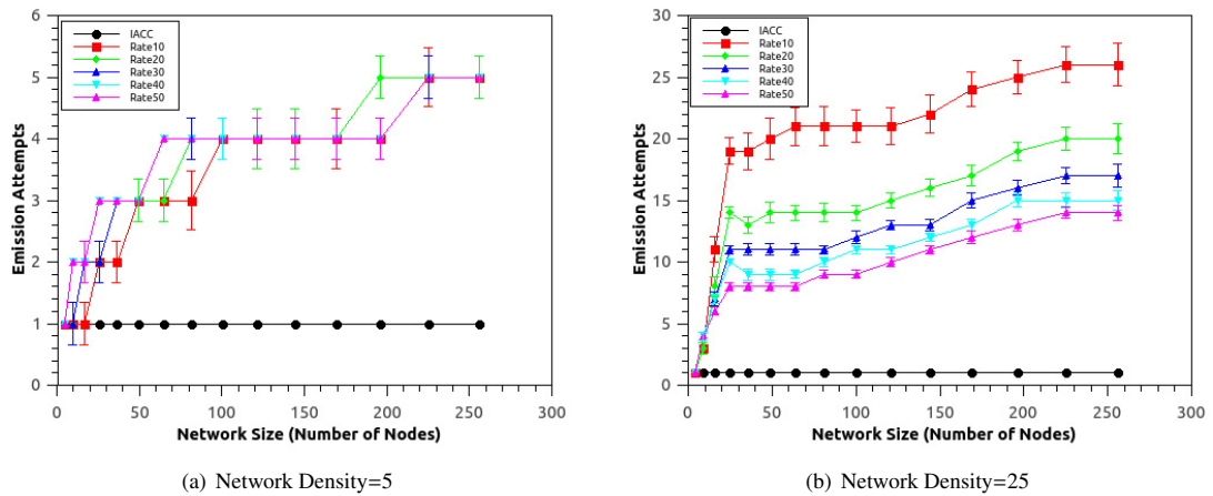
Fig. 3. Emission attempts
