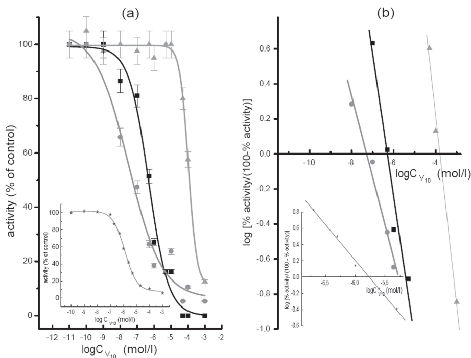
Figure 3. The concentration dependent (a) and Hill analysis (b) inhibition of SPM \text{Na}^+/\text{K}^+ -ATPase (square), \text{Ca}^{2+} -ATPase (circle), \text{Mg}^{2+} -ATPase (triangle) and commercial porcine cerebral cortex \text{Na}^+/\text{K}^+ -ATPase (inset) by ammonium decavanadate ( V_{10} ). C_{V_{10}} , concentration of V_{10} .
