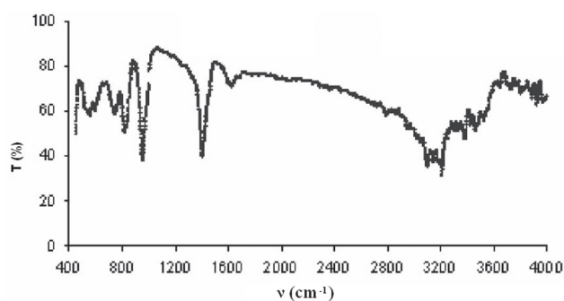
Figure 2. IR spectra (transmittance (T) dependence on wavenumber (v)) of (\text{NH}_4)_6\text{V}_{10}\text{O}_{28} \cdot 5\text{H}_2\text{O} recorded at room temperature.
