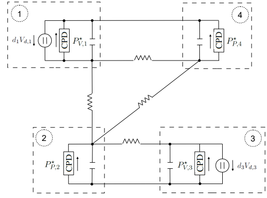
Fig. 2: Four-terminal hvdc transmission system.
