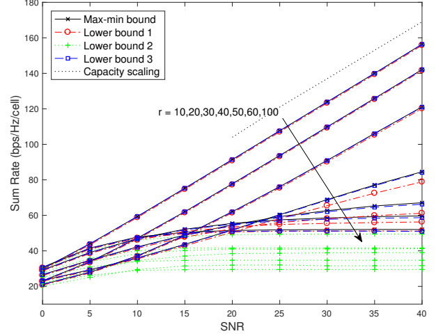
Fig. 1. The impact of spatial despreading on sum-rate scaling with respect to the sparsity of angular supports ( r ), where M = 200, L = 4, K = 10, T_c = 500 . 'Lower bound 1', 'Lower bound 2', and 'Lower bound 3' are given by (5), (6), and (7), respectively. The asymptotic capacity scaling is (8) with o(1) = 0 .
