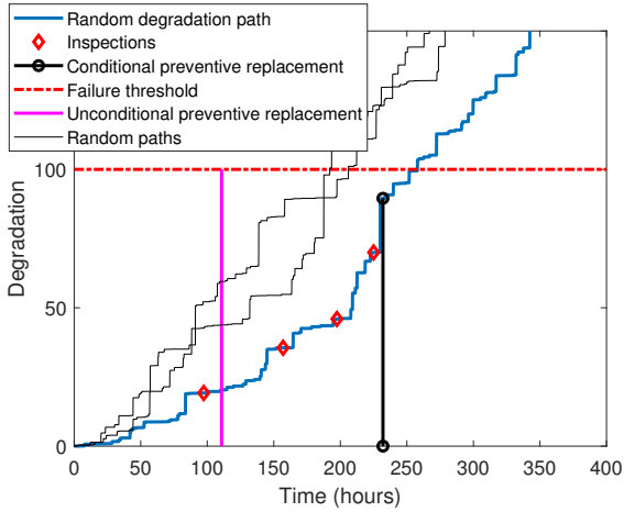
Figure 6: Application of the sequential inspection policy to a random degradation path (thick solid blue line). Other (gamma) degradation 455 paths are also shown (thin solid black lines).
