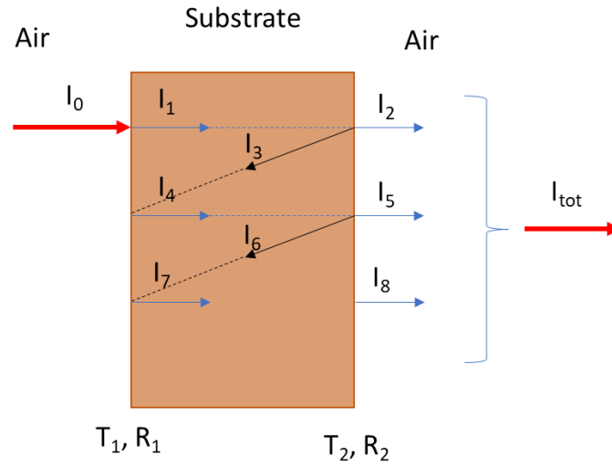
Figure 1: Schematics of the light transmission through a parallel plate substrate in air. The light (intensity I_0 ) comes from the left. The resulting total transmitted light ( I_{tot} ) depends on T_1, R_1, T_2 and R_2
