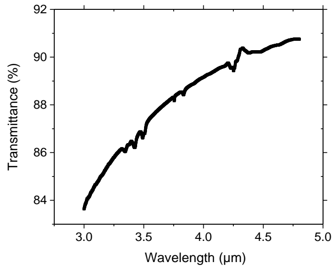
Figure 6: Transmittance spectrum of sample M2 (thickness 1.842mm)
