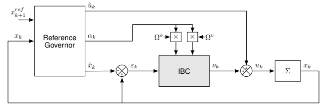
Figure 5: IBT block diagram
