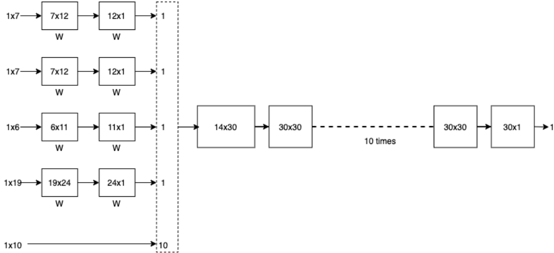
Figure 1: Network Architecture.
